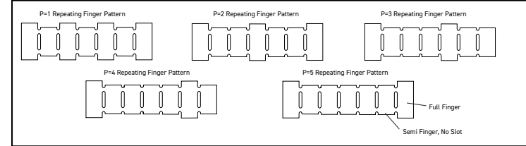
Figure 6 - Variable (Alternating) Slot Mount Configurations
